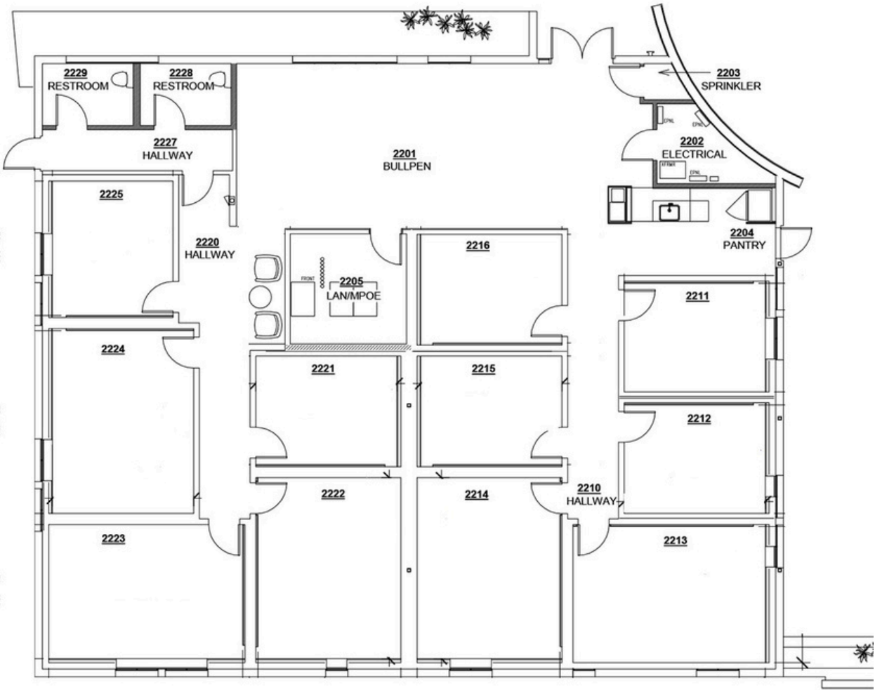
BUILDING 22
